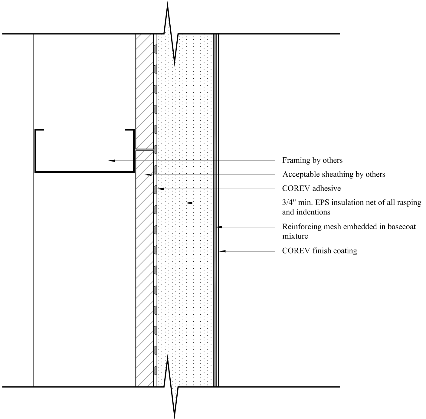
TYPICAL PLAN VIEW
